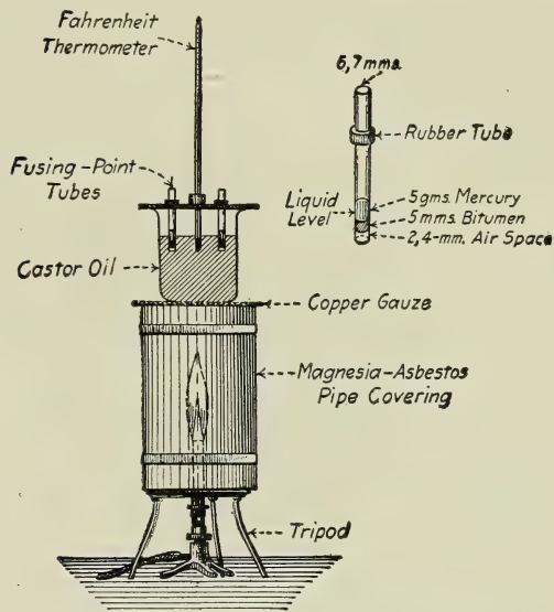
FIG. 176.—K. and S. Tester for High Fusing-Point Substances.
